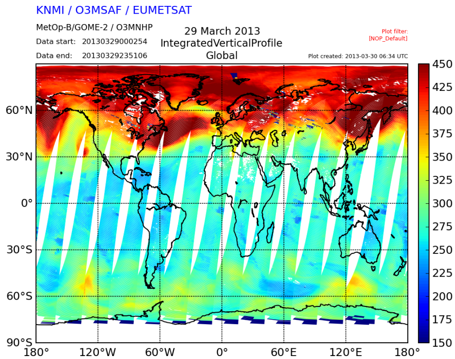
Figure 7.7: Integrated vertical ozone profile from GOME-2 on MetOp-B, calculated as the sum of the retrieved profile on March 29th 2013.
