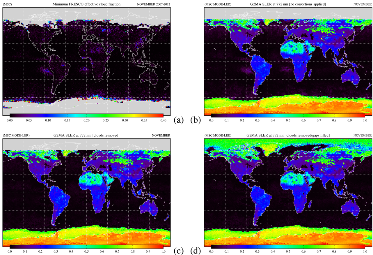
Figure 7: Some intermediate processing results for the month November, determined from GOME-2A observations over the years 2007–2012. (a) Minimum effective FRESKO cloud fraction encountered. (b) Surface LER map showing residual cloud structures over the oceans. (c) Surface LER map after performing the correction for persistent clouds over the oceans. (d) Surface LER map after filling the gaps near the polar regions (due to polar night) with data from other months.
